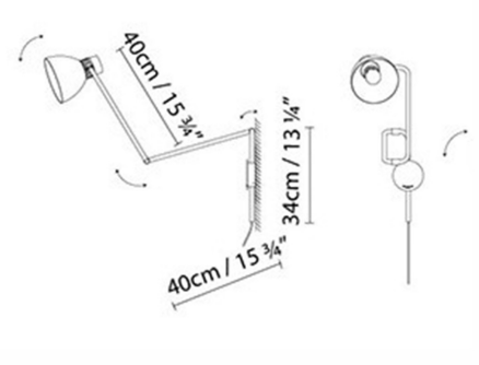
BLUX SYSTEM W40 PLUG-IN
