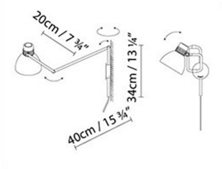
BLUX SYSTEM W20 PLUG-IN
